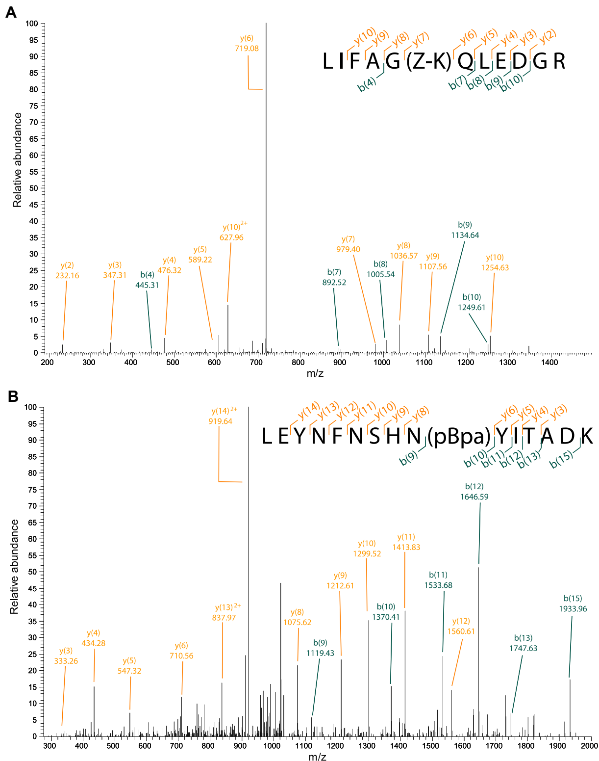
Figure 2. Mass spectral analyzes of tryptic fragments of (A) Ub_K48_Z-lysine and (B) sfGFP_V150_pBpa.
